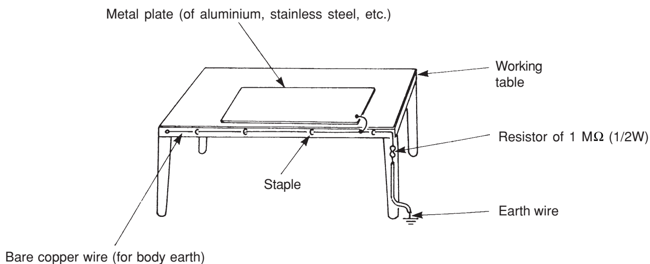
Fig. 3. Grounding of the working table
