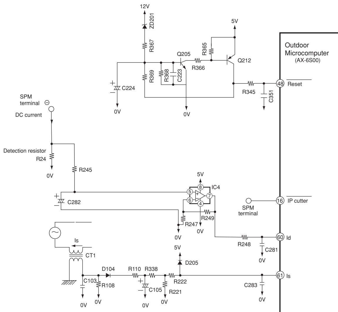
Fig. 7-1 Peripheral circuit of microcomputer (AX-6V)
